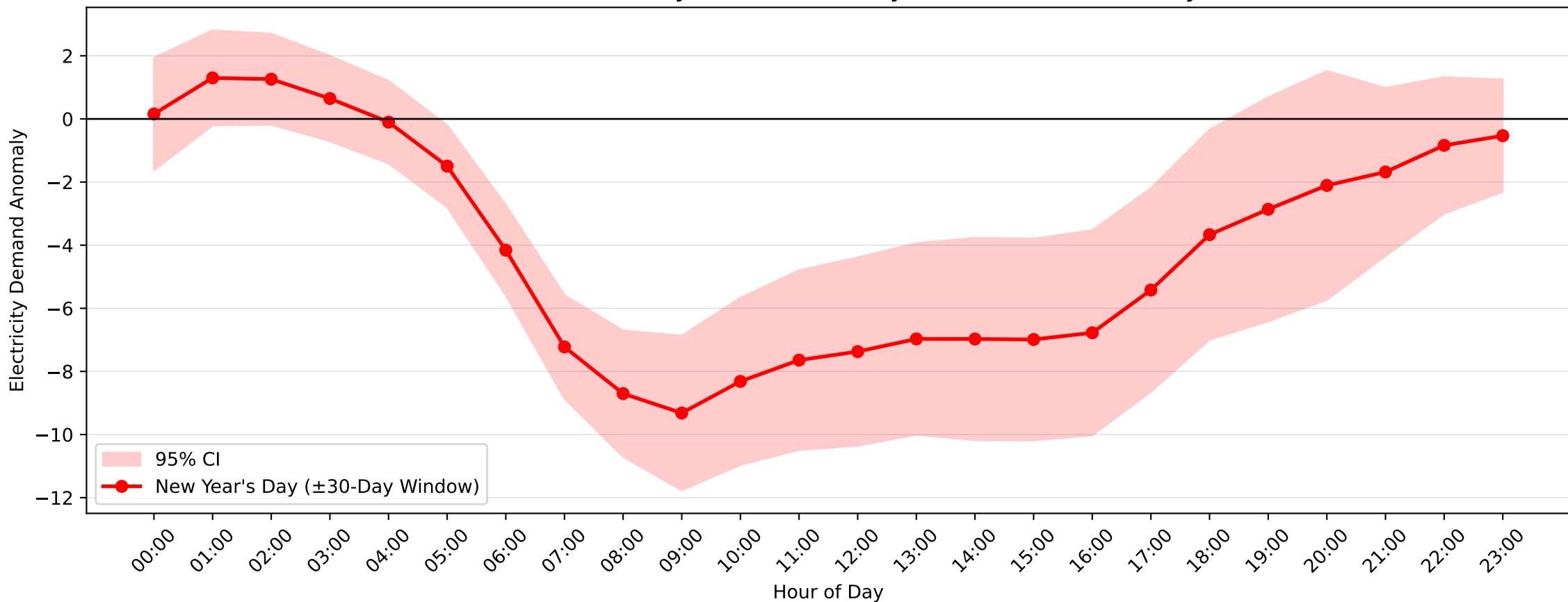
Burwood Demand Anomaly: New Year's Day (2004-2017, \pm 30 -Day Window)
